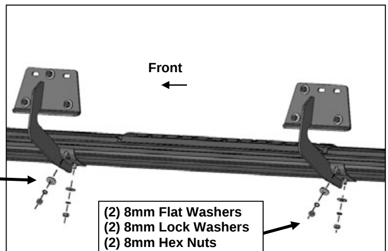
(Fig 8) Passenger/right side Sidebar attached to Mounting Brackets at the center and rear locations
