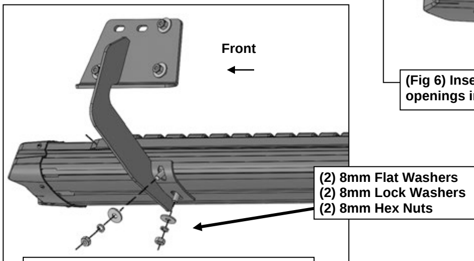
(Fig 7) Passenger side Sidebar attached to Mounting Bracket at the front location
