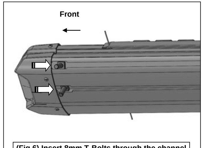
(Fig 6) Insert 8mm T-Bolts through the channel openings in the bottom of the Sidebar
